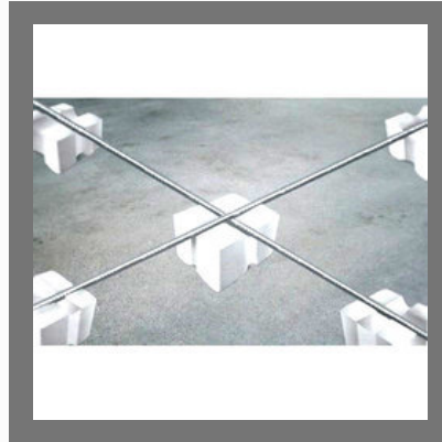
Partition Wall Cover Block
